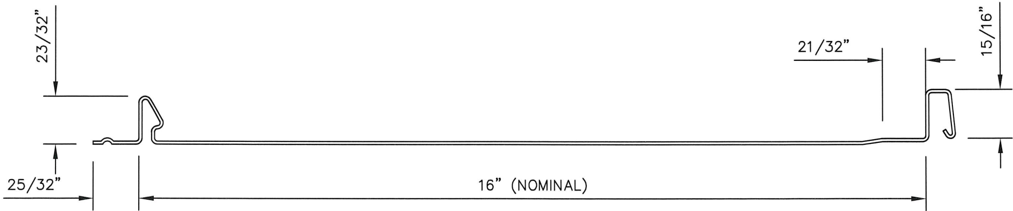
PANEL PROFILE
